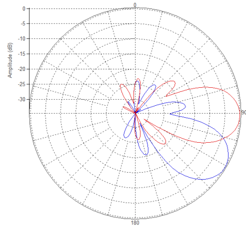
Low-Band Vertical Pattern 0° tilt and 20° tilt (750MHz)
