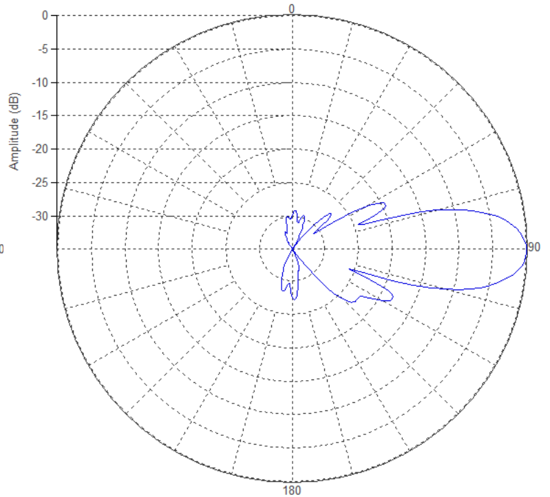
Vertical Pattern (3.95GHz)
