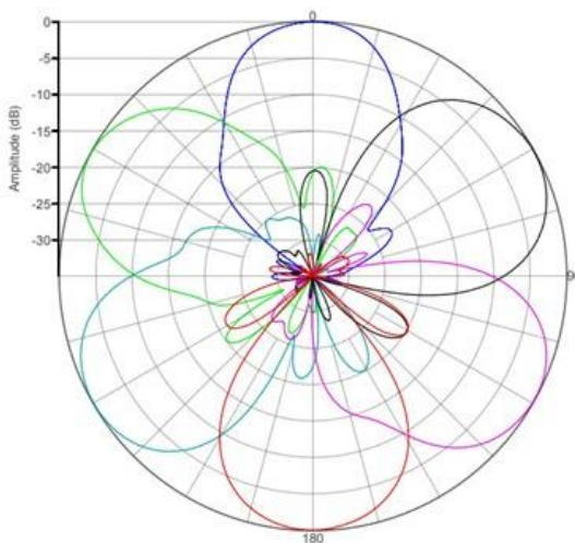
Horizontal Pattern (1.80GHz)
