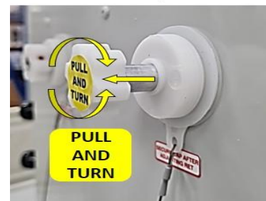
Pull handle out to disengaged RET for tilt adjustment
