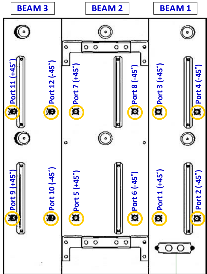
REAR VIEW CONNECTOR LAYOUT
