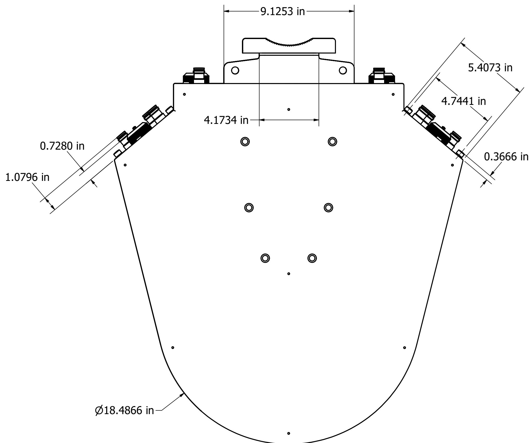
Bottom View
