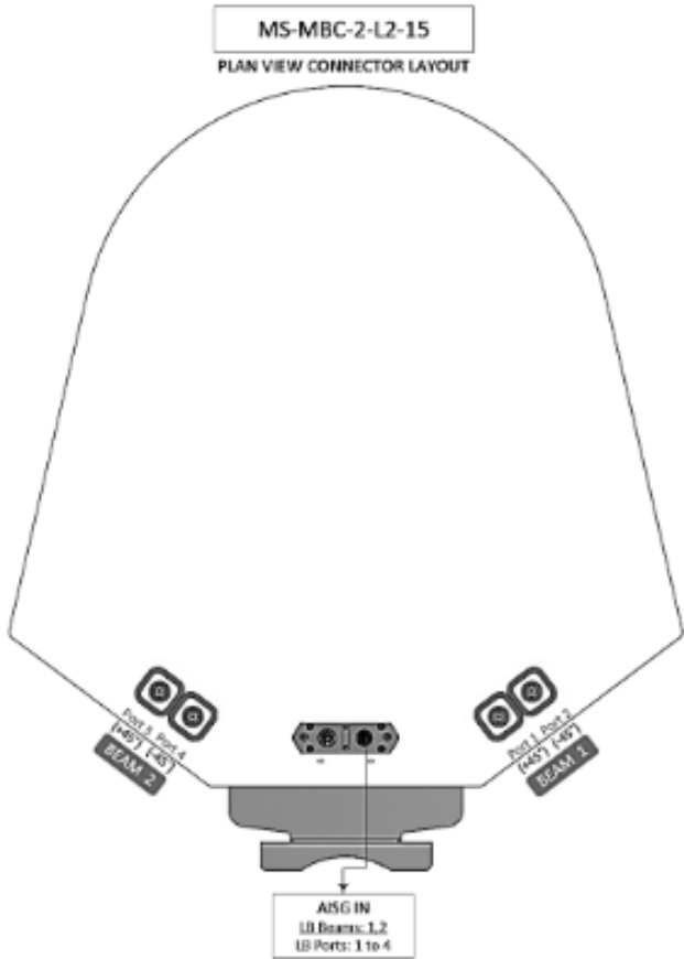
Antenna top view
