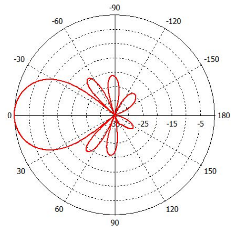
F-Band Vertical pattern (3.5GHz) at tilt 0°
