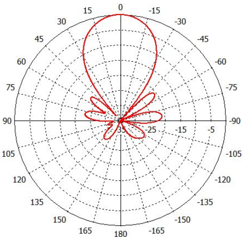
High-Band Horizontal Pattern (1.92GHz)
