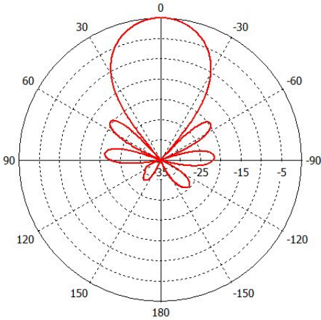
F-Band Horizontal Pattern (3.5GHz)
