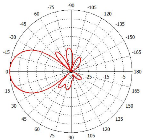
High-band Vertical Pattern (1.92GHz) at tilt 0°
